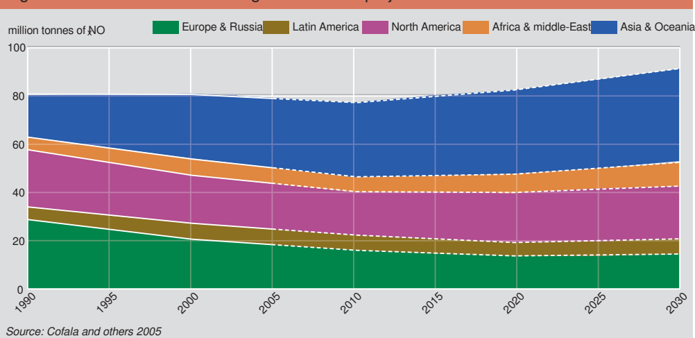
Figure 8: Global emissions of nitrogen oxides and projections
