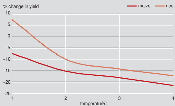
Figure 4: Maize and rice yields versus temperature increase in the tropics averaged across 13 crop modelling studies
