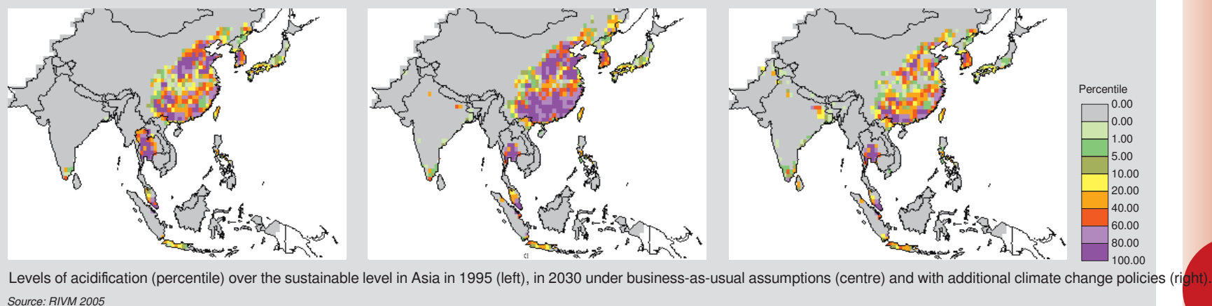
Figure 6: Acidification risks in Asia
