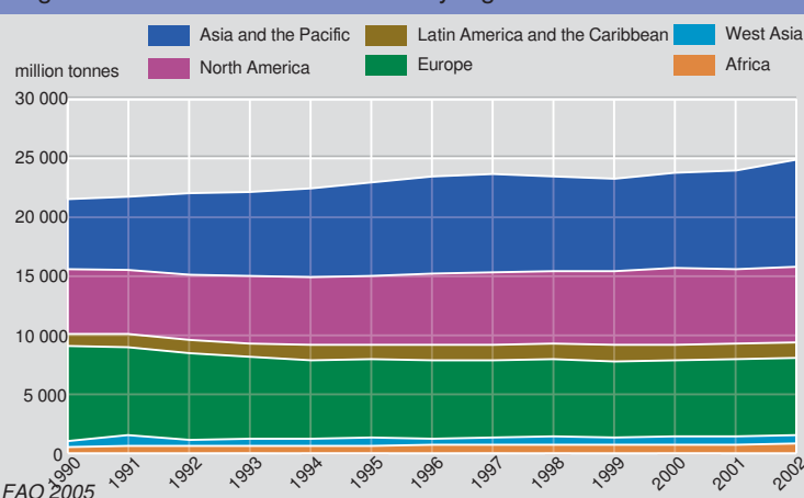
Figure 4: Carbon dioxide emissions by region
