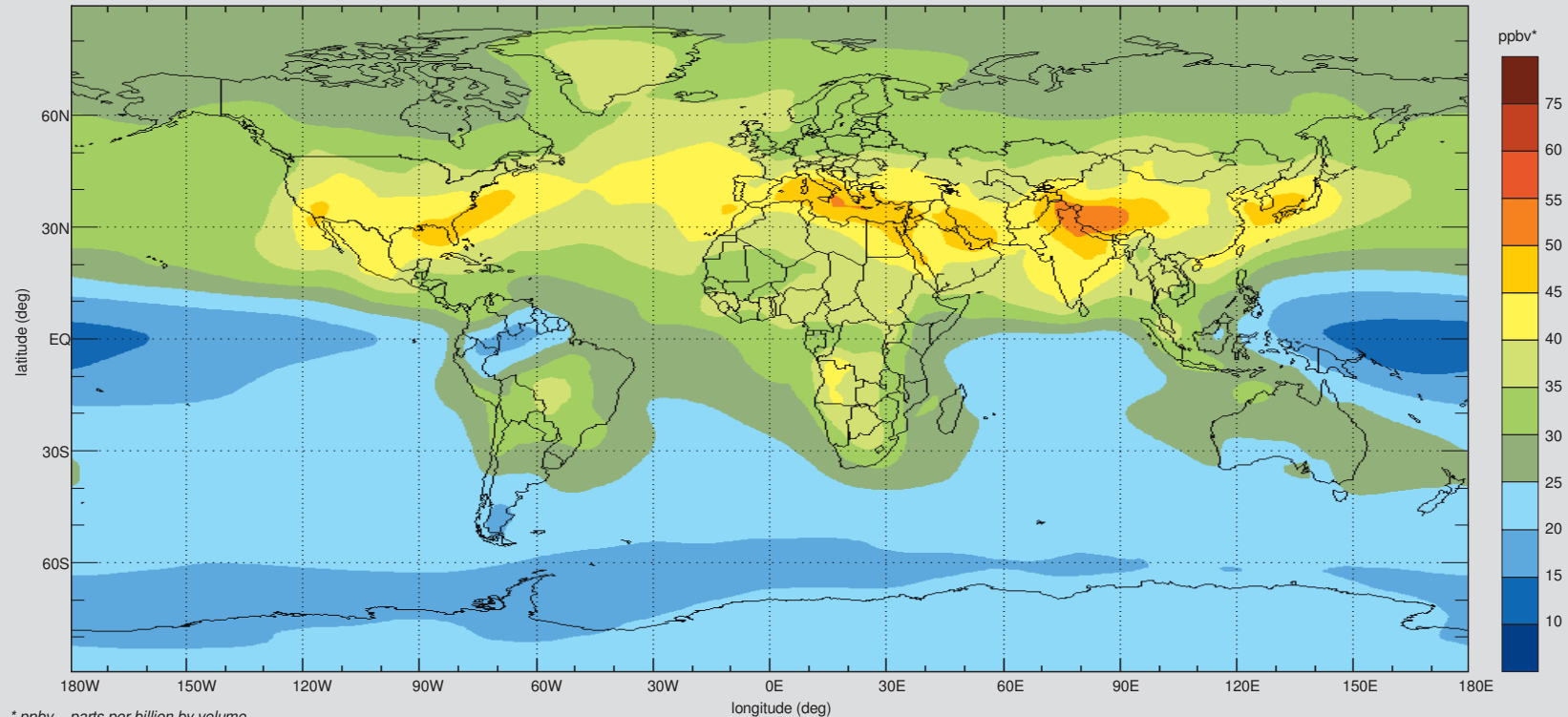
Figure 9: Annual average of surface ozone in 2000
