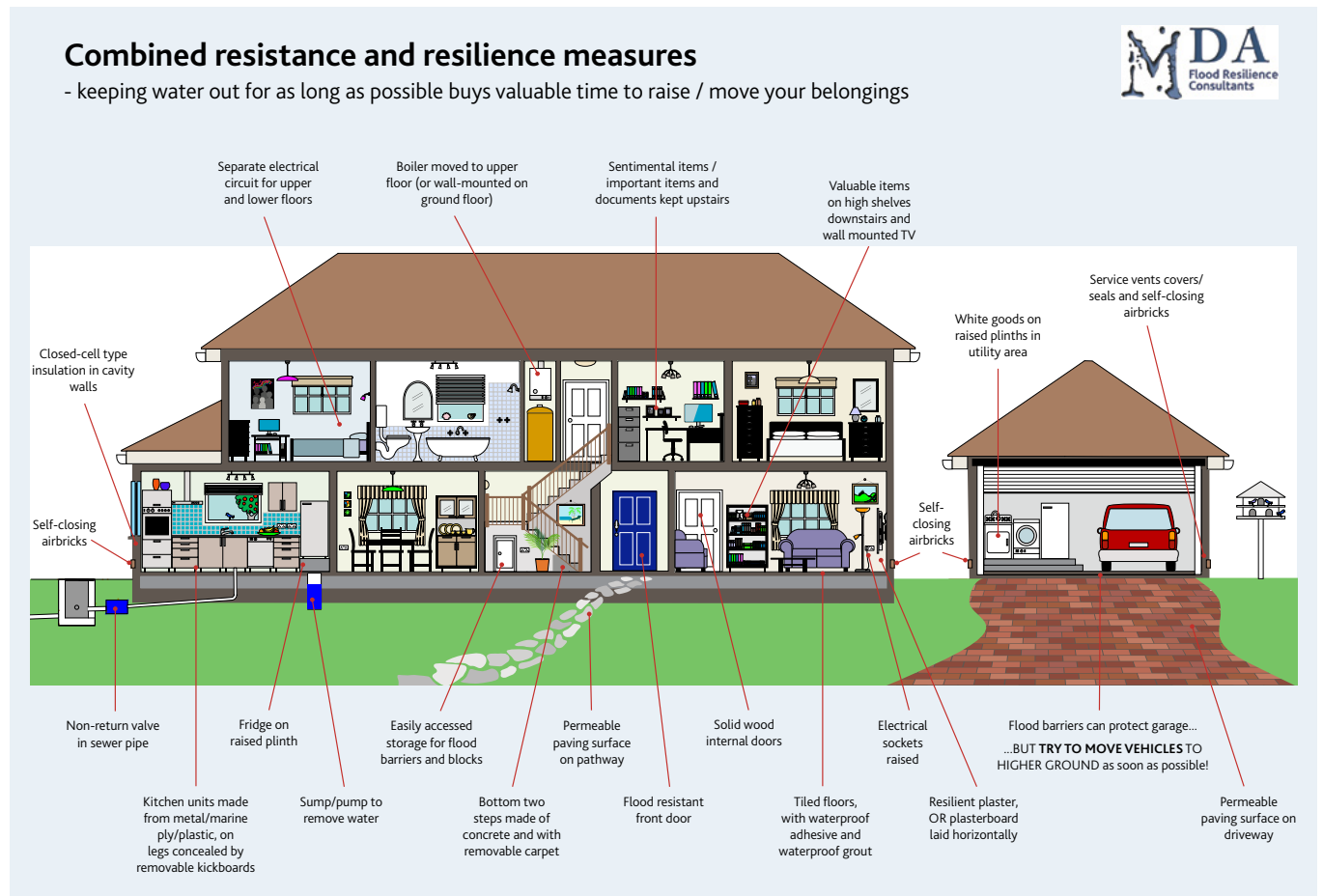
Source: Lamond et al. 2018. Evidence review for property flood resilience phase 2. Illustration: Mary Dhonau, MDA Flood Resilience Consultants (65)
